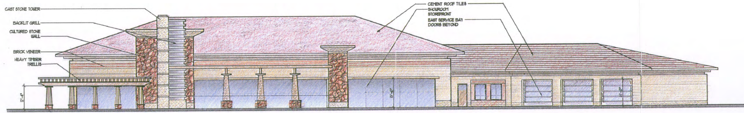
4 EAST ELEVATION SCALE: 1/16" = 1'-0"
