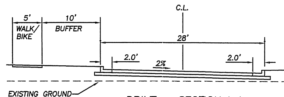
DRIVE - SECTION I-I
