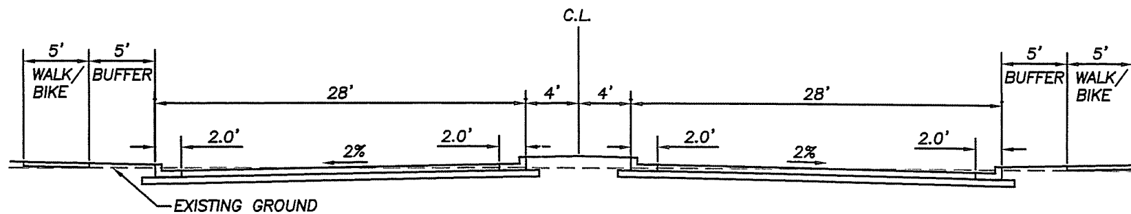
DRIVE - SECTION F-F
