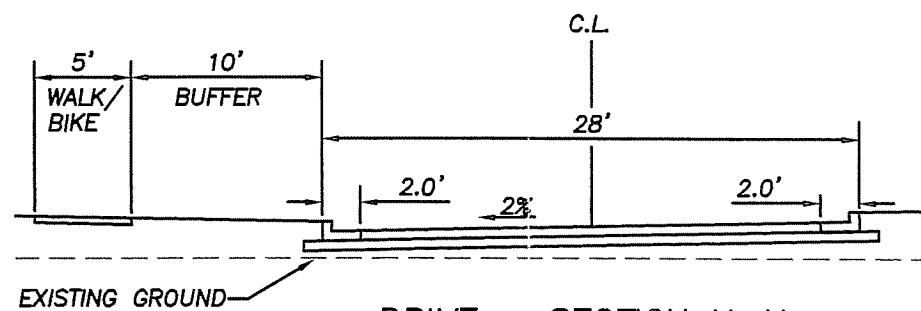
DRIVE - SECTION H-H
