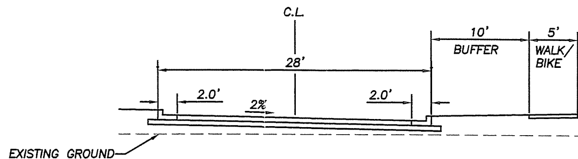
DRIVE - SECTION G-G
