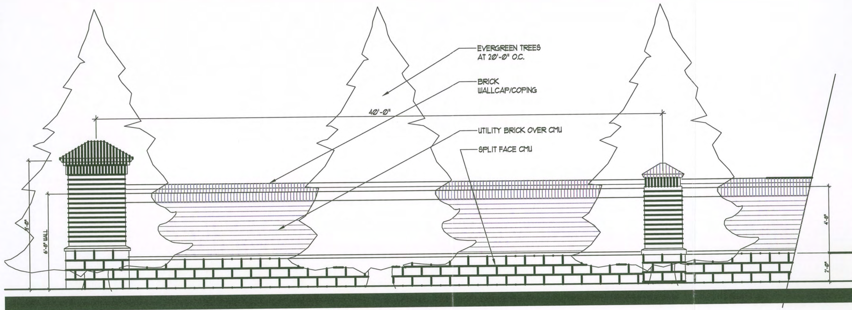
1 CONCEPTUAL ELEVATION AI-01 SCALE: 1/4" = 1'-0"
