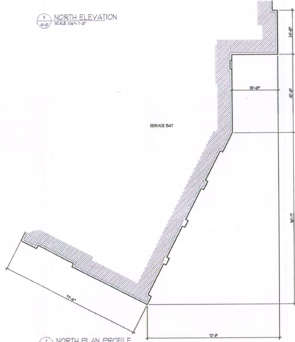
2 NORTH PLAN PROFILE SCALE: 1/16" = 1'-0"
